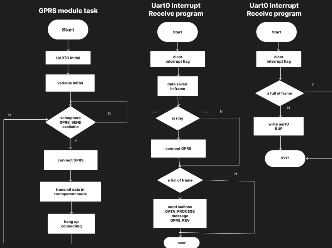
The operation of General Packet Radio Service (GPRS)
